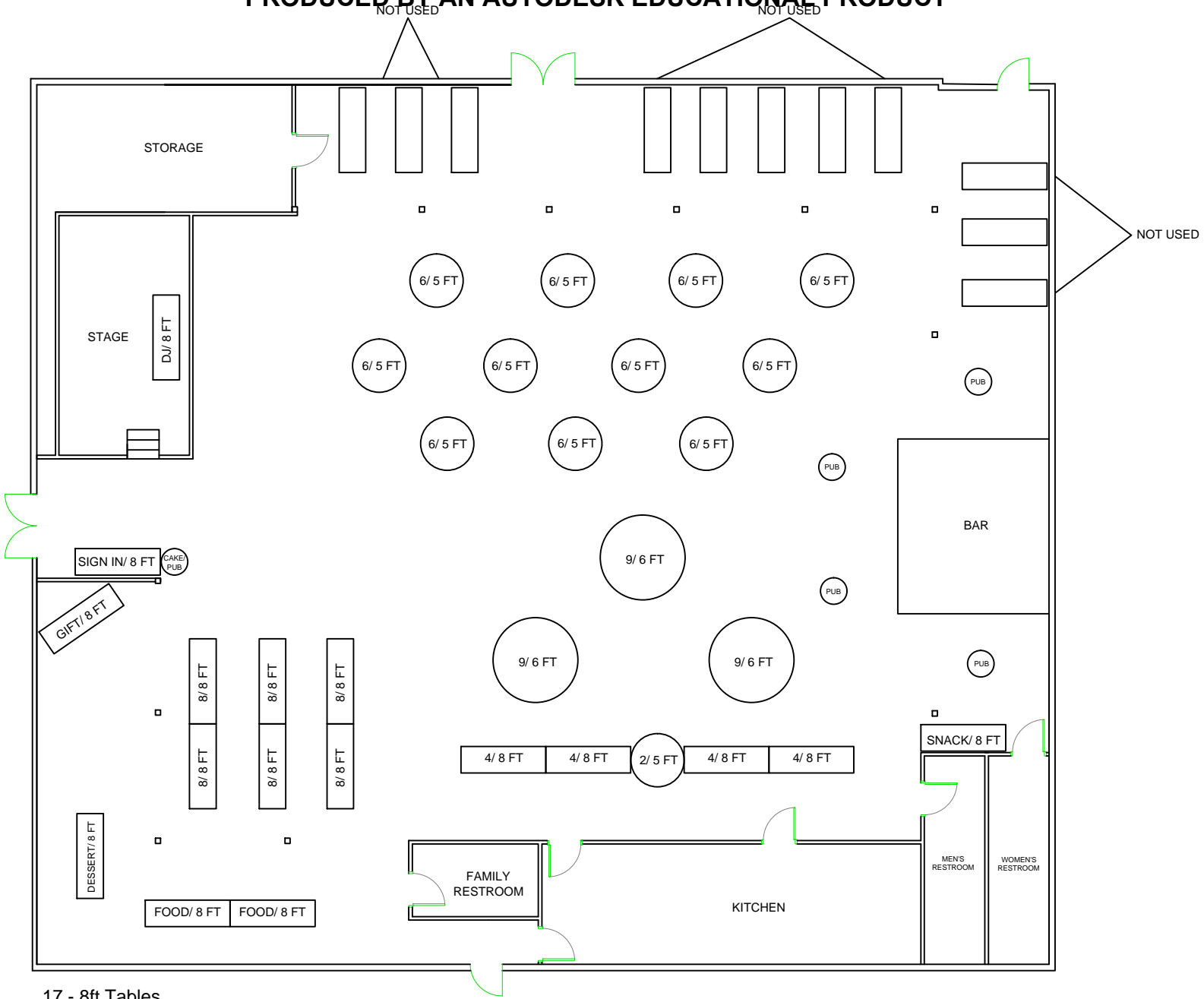
150 Person Layout/Actual 159
